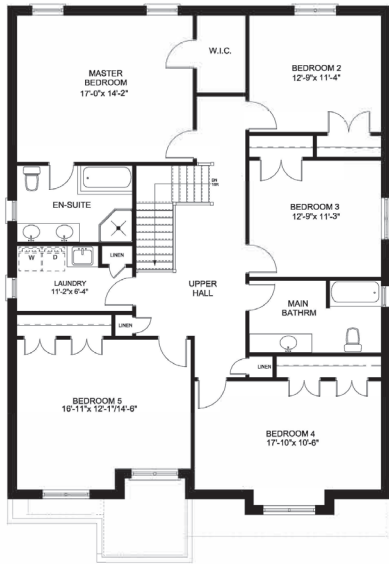
SECOND FLOOR 1,695sf 5 BEDROOM OPTION
