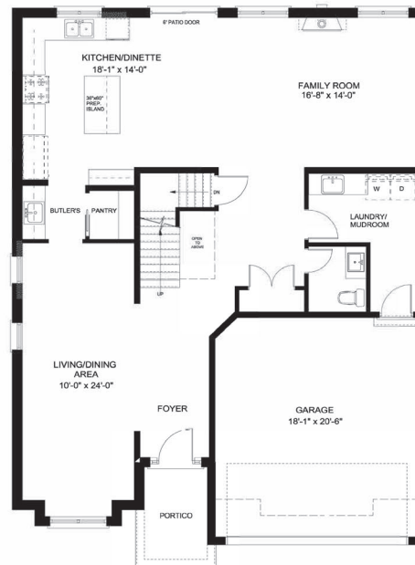
GROUND FLOOR PLAN 1,374sf
