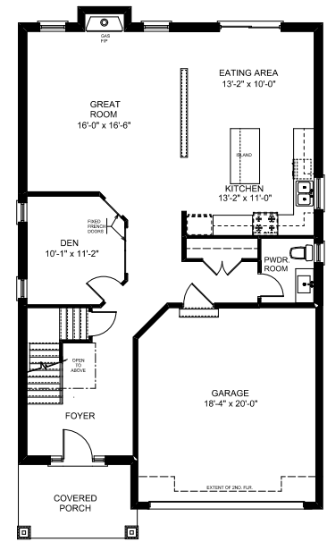
Alternate Ground Floor 1121sf
